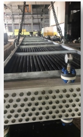
Air Cooler Fabrication - Offshore Vietnam
